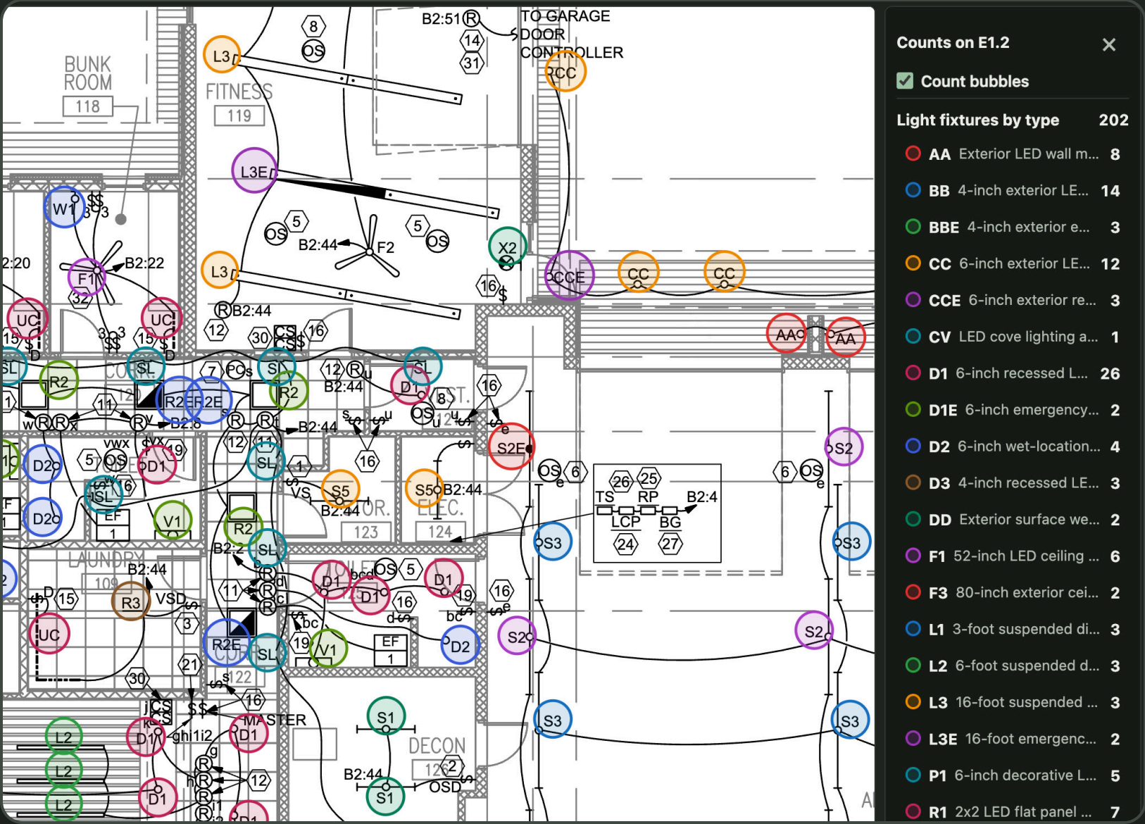
Lighting plan: light fixtures by type, counted beside the sheet
